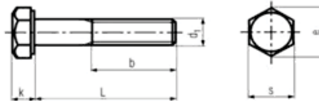
HEX BOLT
