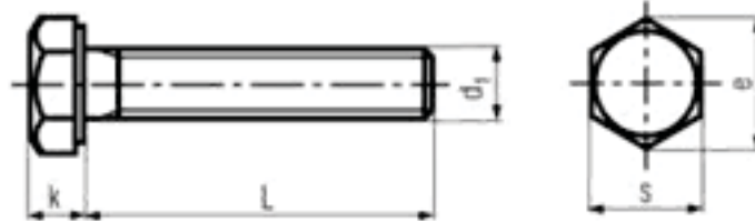
HEX SCREW
